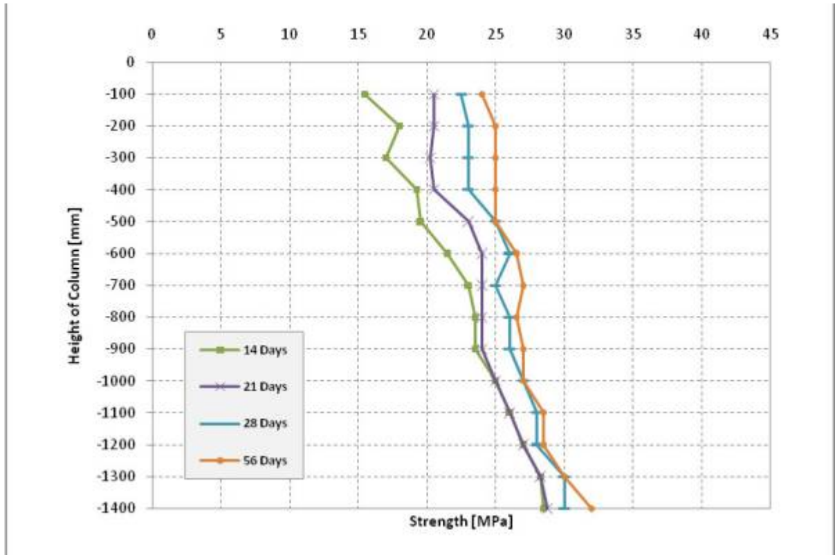
Figure C6: Column C6 - Cardboard Tube, Normal Concrete.
