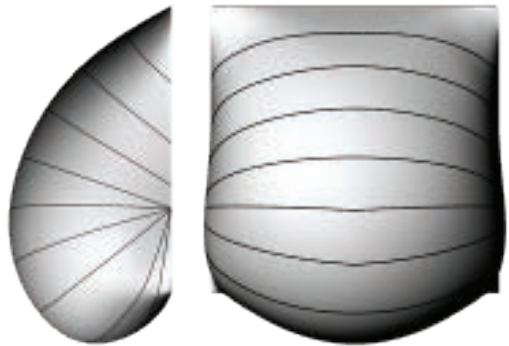
Figure 14: Possible patterns of the final geometry based on geodesic lines between points along the boundaries.
